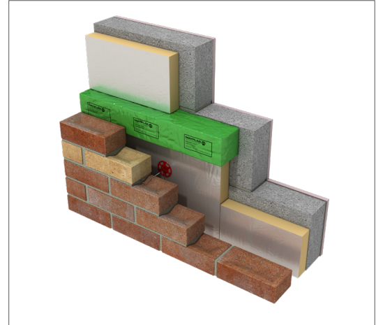
MP552 Masonry Cavity Barrier - mid-cavity (construction by others)
