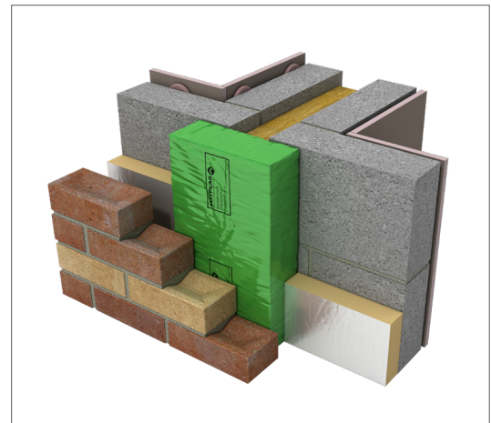
MP552 Masonry Party Wall Barrier - installed vertically (construction by others)
