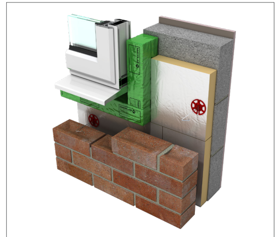
MP552 Masonry Cavity Barrier - around aperture (construction by others)
